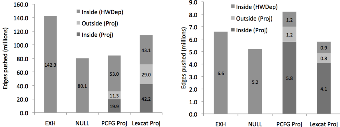
Figure 4: Comparison between a CKY simulation (EXH), A* with no heuristic (NULL), hierarchical A* (HA*) using two grammar projections for standard search (left) and AST (right). The breakdown of the inside/outside edges for the grammar projection as well as the target grammar shows that the projections, serving as the heuristic estimates for the target grammar, are costly to compute.
